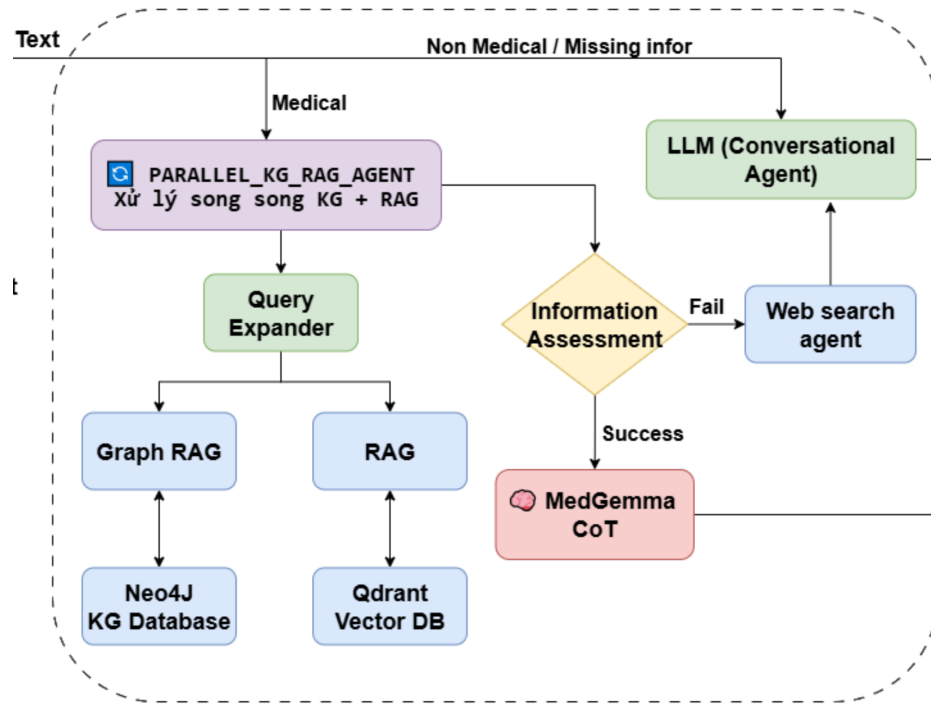
Figure 3.3: Text Module architecture for medical knowledge retrieval
